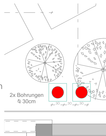
0. Position Kamin 1:50
